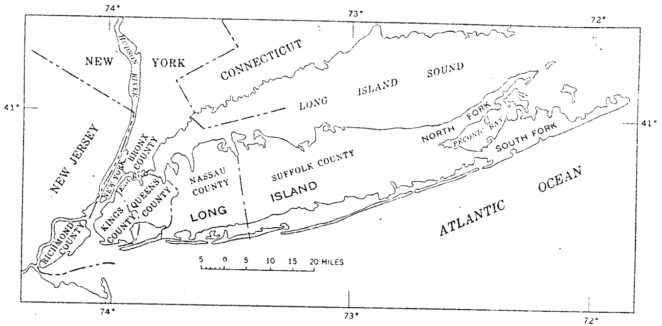
Figure 1.—Long Island and vicinity.
